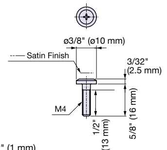
Screw M4x16
