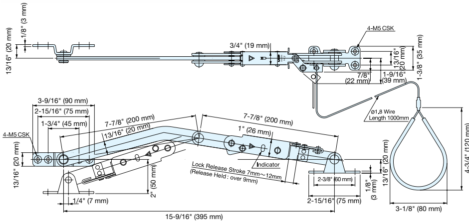
Installation of lock-release wire (WR and WL type only)
