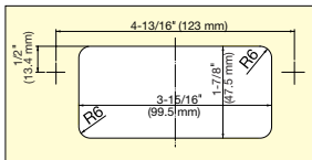
Bore Dimensions
