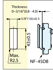
Sheet metal
