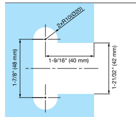
Bore Dimensions
