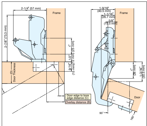
Bore Dimensions
