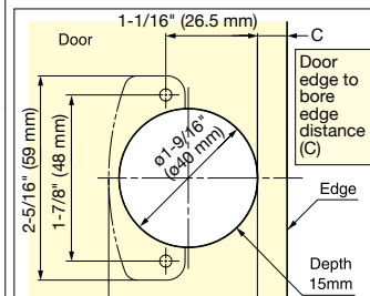
Bore Dimensions
