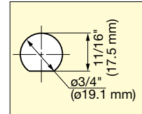
Cut Out Dimensions (Master Key Type)
