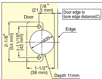
Bore Dimensions
