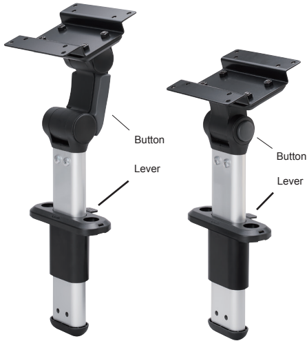
Dual axis type
