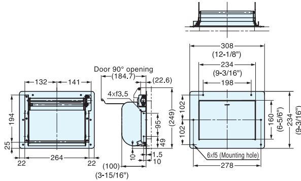
Cut Out Dimensions
