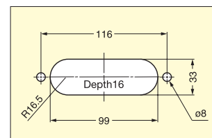
Bore Dimensions
